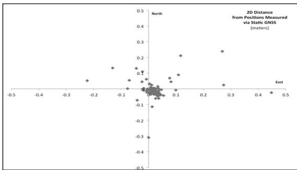
Plot of CenterPoint RTX via static GNSS positions. Accuracy of 5cm or better was common.
